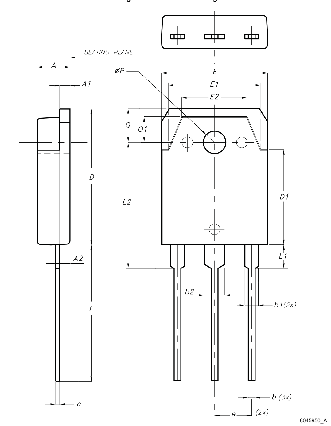
Figure 36. TO-3P drawing
