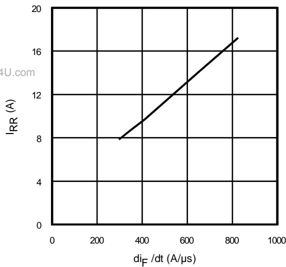
Fig. 19 - Typical Diode I RR vs. di F /dt V CC = 400V; V GE = 15V; I CE = 5.0A; T J = 150°C
