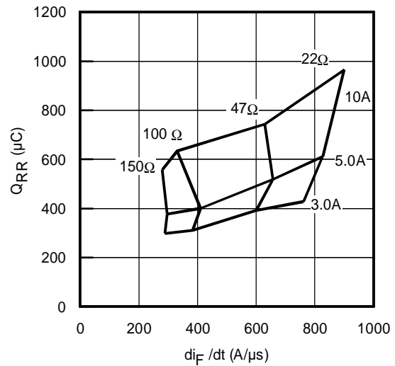
Fig. 20 - Typical Diode Q RR V CC = 400V; V GE = 15V; T J = 150°C
