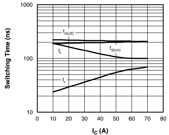
Fig. 10 - Typical IGBT Switching Time vs. I_C T_J = 125 \text{ }^\circ\text{C} , L = 500 \text{ } \mu\text{H} , V_{CC} = 360 V , R_g = 5 \text{ } \Omega , V_{GE} = 15 V
