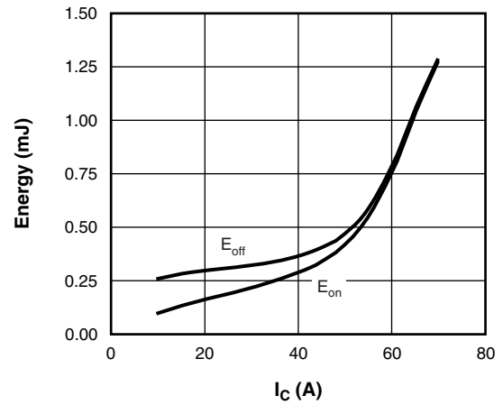
Fig. 9 - Typical IGBT Energy Loss vs. I_C T_J = 125 \text{ }^\circ\text{C} , L = 500 \text{ } \mu\text{H} , V_{CC} = 360 V , R_g = 5 \text{ } \Omega , V_{GE} = 15 V
