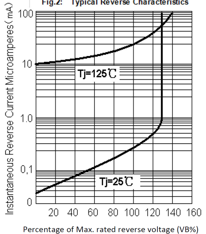
Fig.2: Typical Reverse Characteristics
