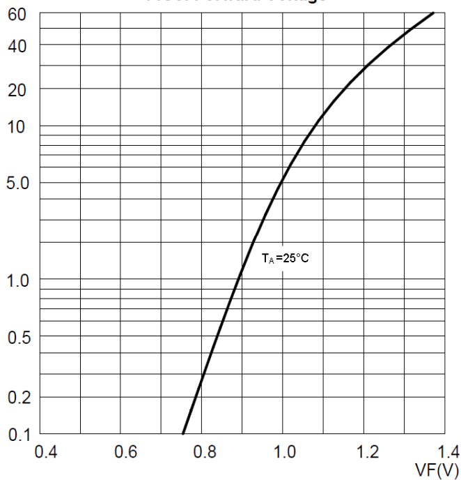
FIG3: Forward Voltage
