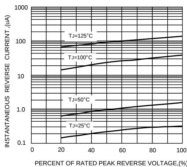
FIG.5-TYPICAL REVERSE CHARACTERISTICS
