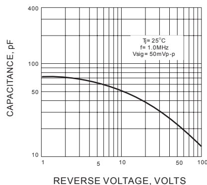
Fig.2 - TYPICAL JUNCTION CAPACITANCE PER ELEMENT
