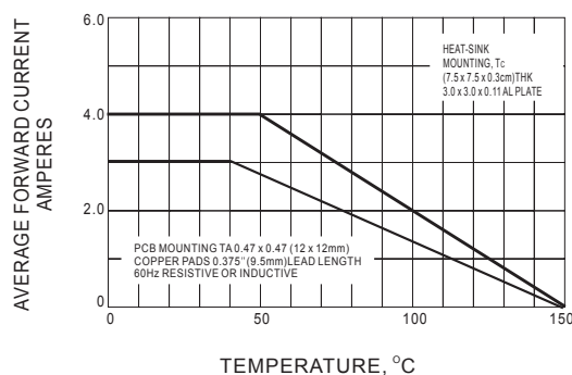
Fig.1 - DERATING CURVE FOR OUTPUT RECTIFIED CURRENT
