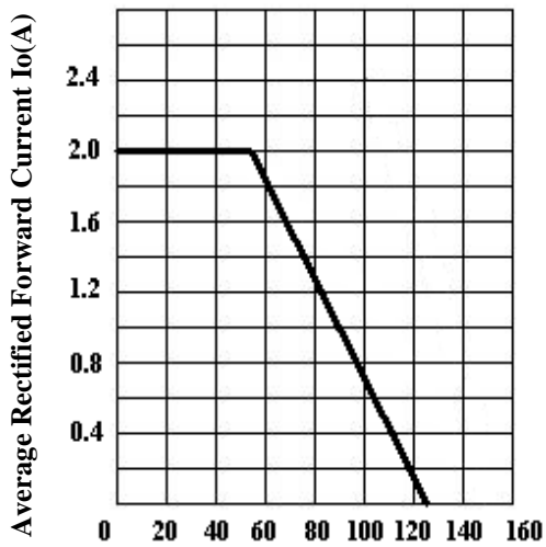
Fig.1 derating Curve
