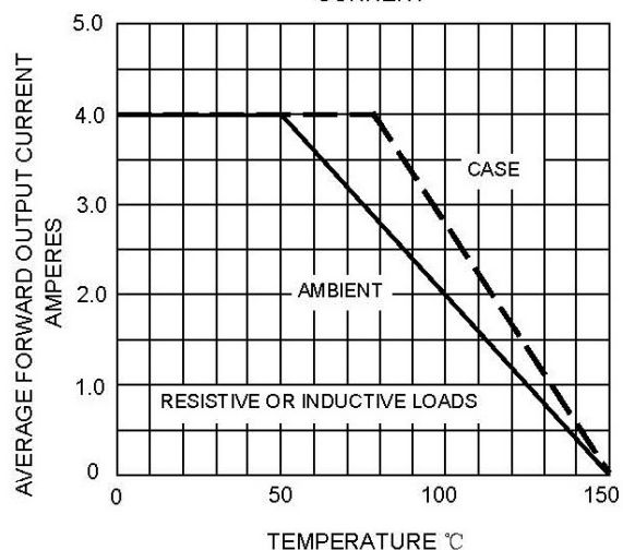
FIG.2-FORWARD DERATING CURRENT
