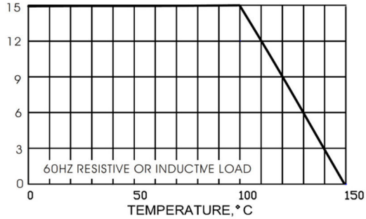
FIG.1-DERATIVE CURVE FOR OUTPUT RECTIFIER CURRENT
