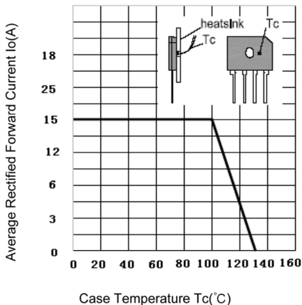
Fig. 1 Derating Curve
