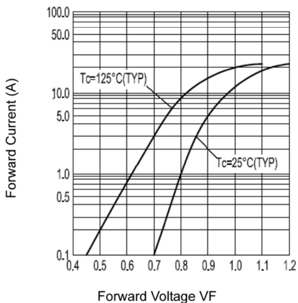
Fig.3 Forward Voltage
