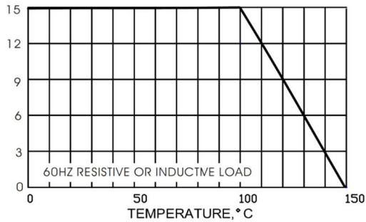
FIG.1-DERATIVE CURVE FOR OUTPUT RECTIFIER CURRENT
