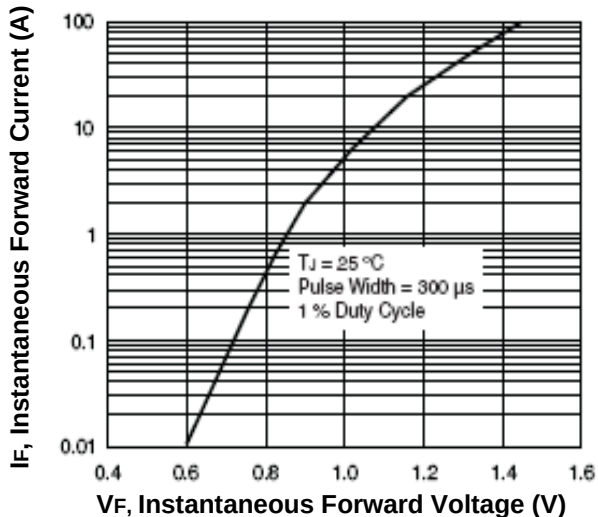
Fig.3-Typical Forward Characteristic per leg
