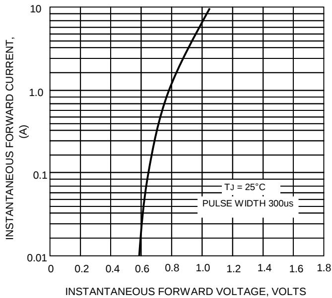
FIG.4-TYPICAL FORWARD CHARACTERISTICS
