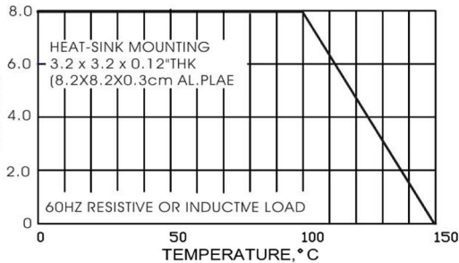
FIG.1-DERATIVE CURVE FOR OUTPUT RECTIFIER CURRENT
