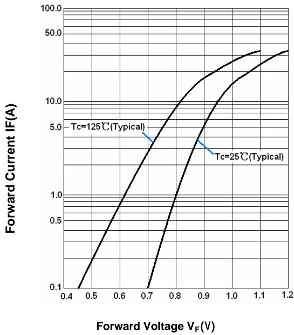
Fig.4 Forward Voltage
