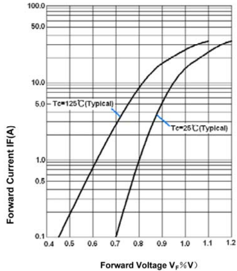
Fig.4 Forward Voltage
