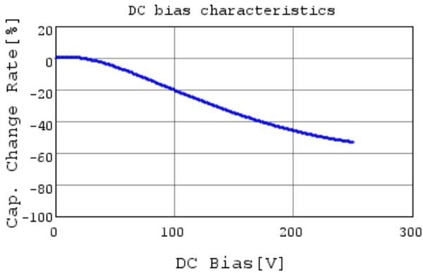
GC321AD72E103KX01 C-DC bias capchange, 25.0c
