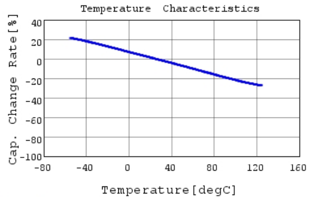
GC321AD72E153KX01 C-Temp. capchange, DCOV, 1
