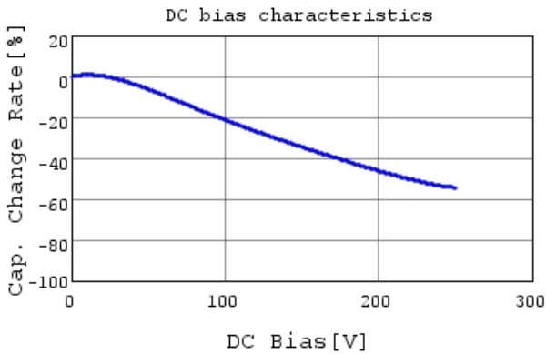
GC321AD72E153KX01 C-DC bias capchange, 25.0c
