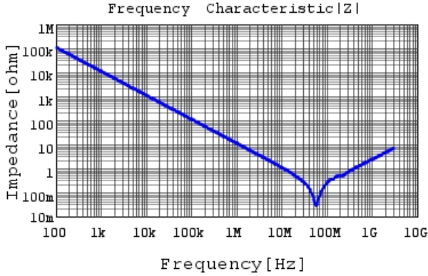
GC321AD72E153KX01 |Z| DCOV, 25degC
