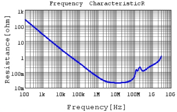
GC321AD72E153KX01 R DCOV, 25degC
