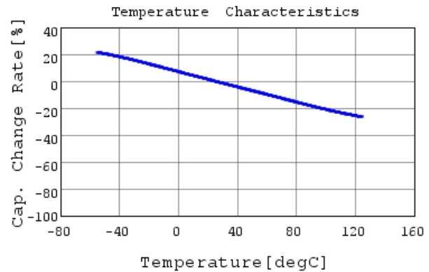
GC321BD72E223KX03 C-Temp. capchange, DCOV, 1
