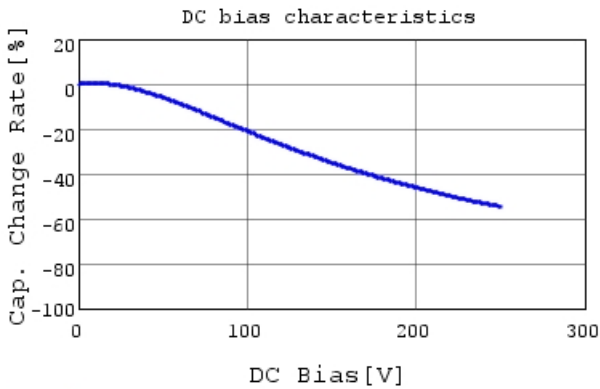
GC321BD72E223KX03 C-DC bias capchange, 25.0c
