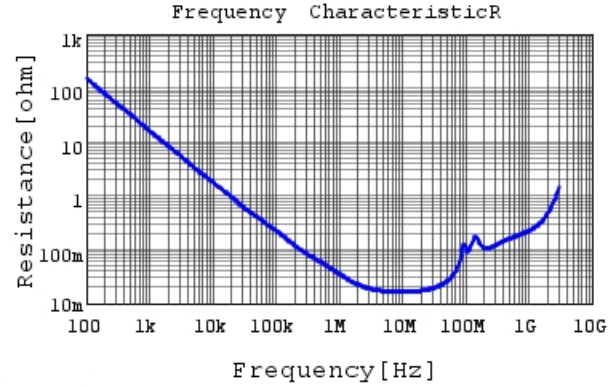
GC321BD72E223KX03 R DCOV, 25degC
