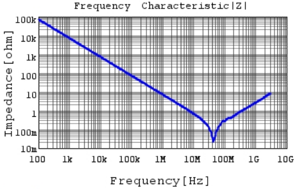
GC321BD72E223KX03 |Z| DCOV, 25degC
