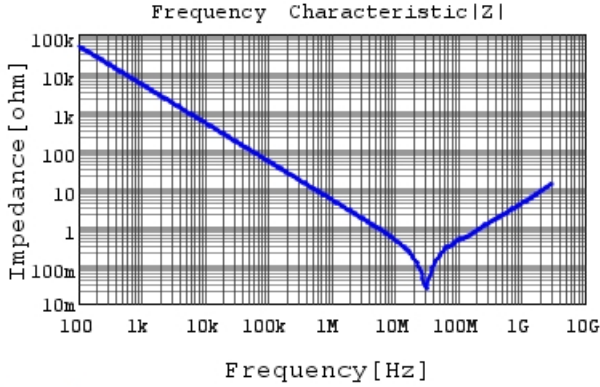
GC331AD72E333KX01 |Z| DCOV, 25degC
