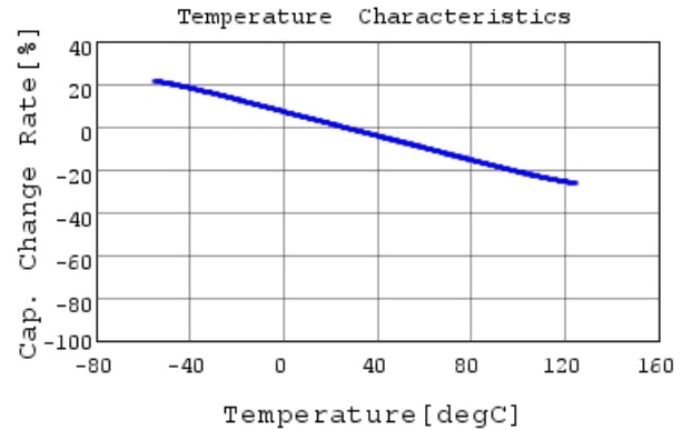
GC331AD72E333KX01 C-Temp. capchange, DCOV, 1
