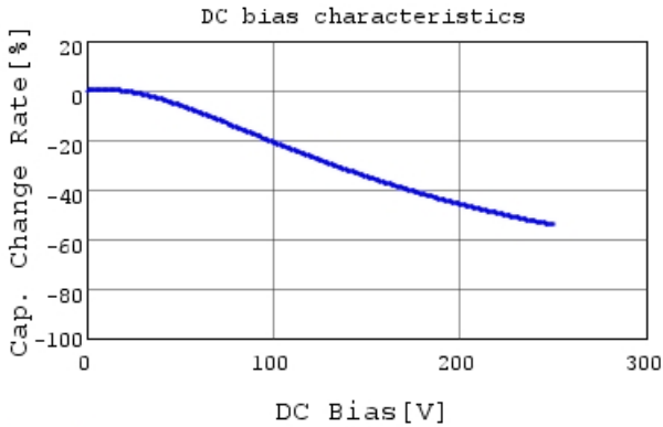
GC331AD72E333KX01 C-DC bias capchange, 25.0c
