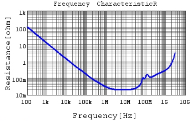
GC331AD72E333KX01 R DCOV, 25degC
