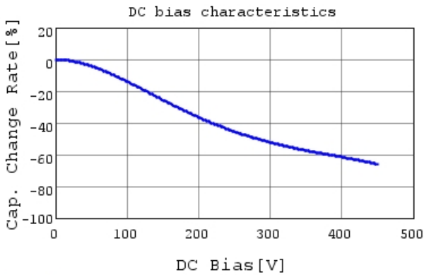
GC331AD72W153KX01 C-DC bias capchange, 25.0c
