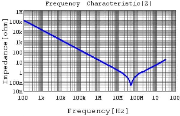
GC331AD72W153KX01 |Z| DCOV, 25degC
