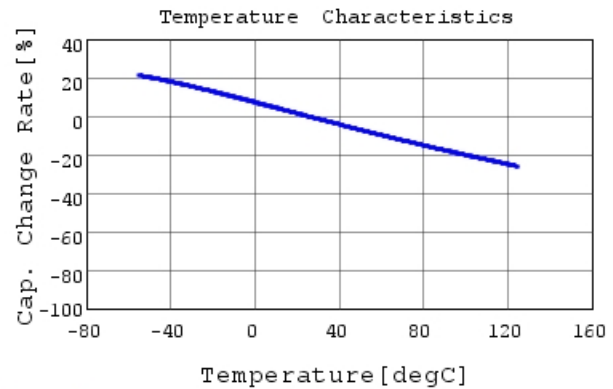
GC331AD72W153KX01 C-Temp. capchange, DCOV, 1
