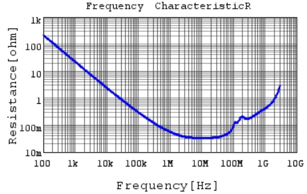
GC331AD72W153KX01 R DCOV, 25degC
