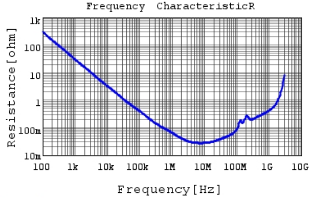
GC331BD72J103KX01 R DCOV,25degC
