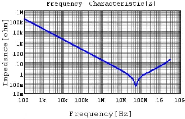
GC331BD72J103KX01 |Z| DCOV,25degC
