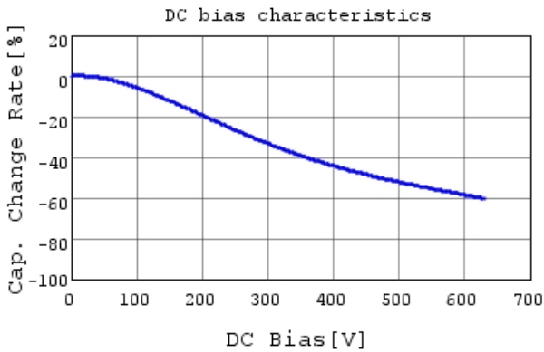
GC331BD72J103KX01 C-DC bias capchange, 25.0c
