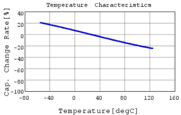
GC331BD72J103KX01 C-Temp. capchange, DCOV, 1
