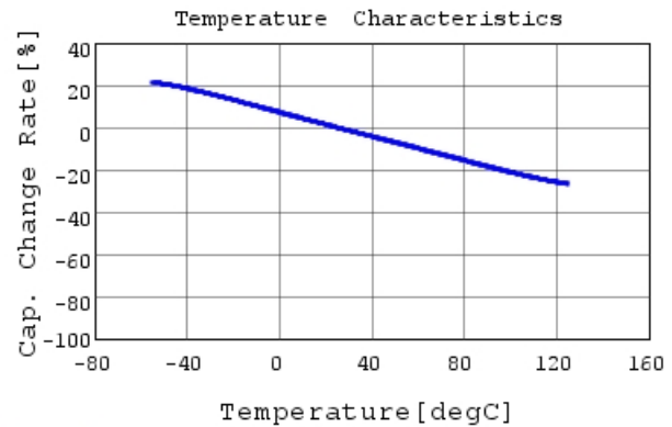
GC331BD72W223KX01 C-Temp. capchange, DCOV, 1
