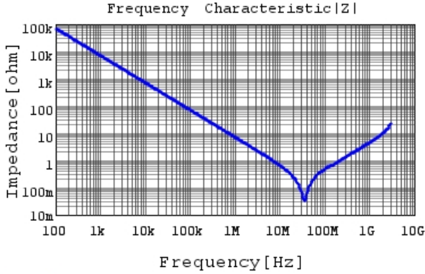
GC331BD72W223KX01 |Z| DCOV, 25degC
