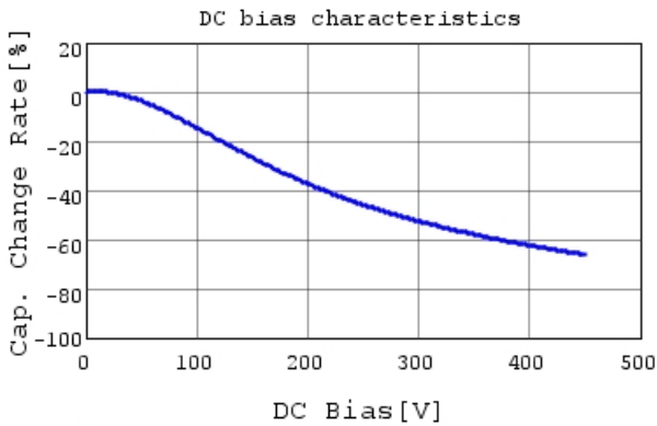
GC331BD72W223KX01 C-DC bias capchange, 25.0c
