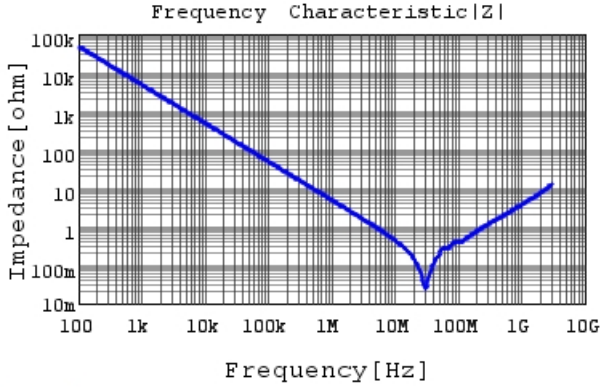
GC331BD72W333KX01 |Z| DCOV, 25degC
