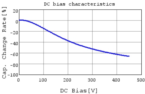
GC331BD72W333KX01 C-DC bias capchange, 25.0c
