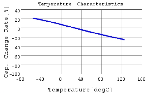
GC331BD72W333KX01 C-Temp. capchange, DCOV, 1
