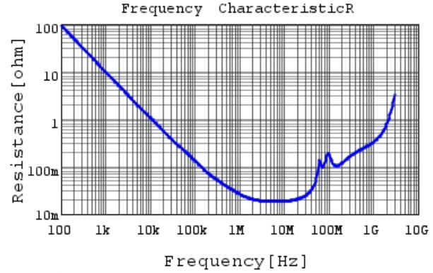
GC331BD72W333KX01 R DCOV, 25degC
