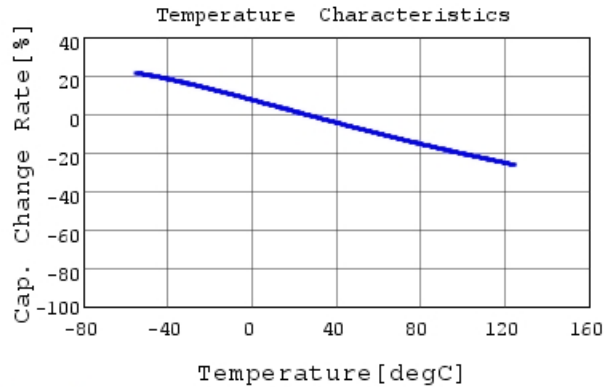
GC331CD72J153KX03 C-Temp. capchange, DC0V, 1
