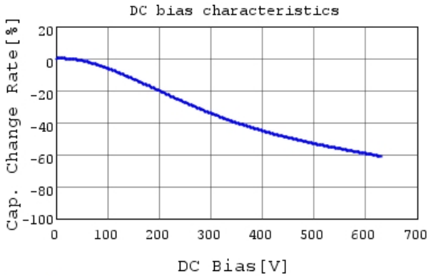
GC331CD72J153KX03 C-DC bias capchange, 25.0c
