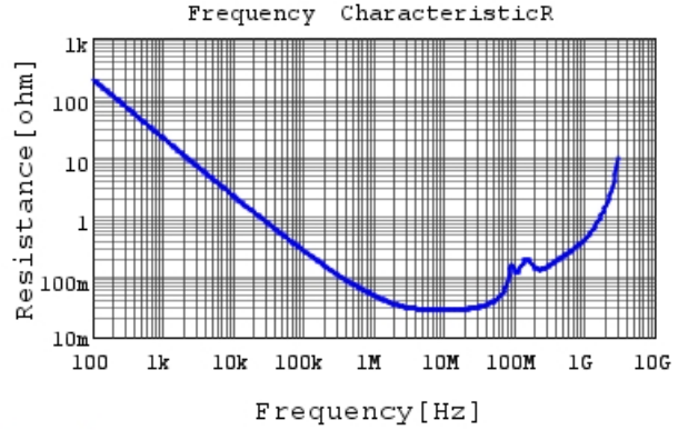
GC331CD72J153KX03 R DC0V, 25degC
