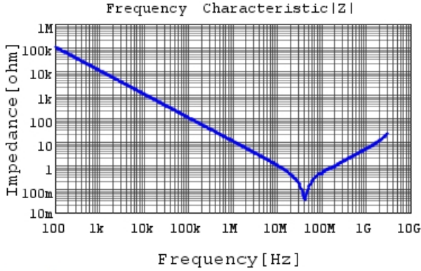
GC331CD72J153KX03 |Z| DC0V, 25degC
