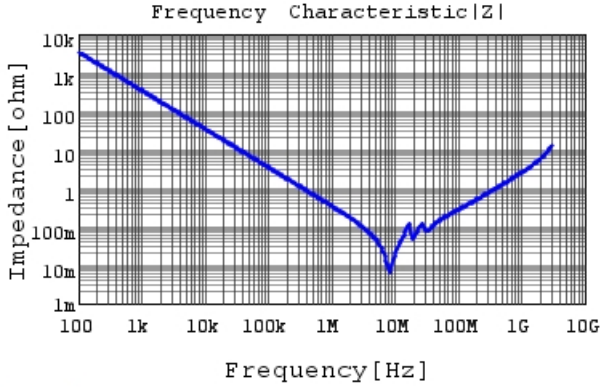
GC355DD72E474KX01 |Z| DCOV, 25degC
