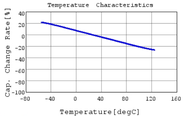
GC355DD72E474KX01 C-Temp. capchange, DCOV, 1
