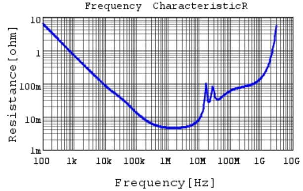
GC355DD72E474KX01 R DCOV, 25degC
