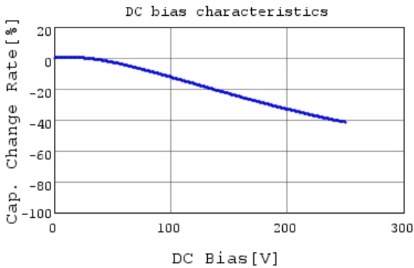
GC355DD72E474KX01 C-DC bias capchange, 25.0c
