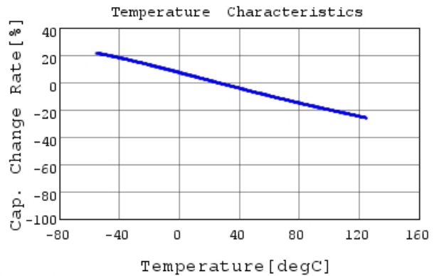
GC355DD72J104KX01 C-Temp. capchange, DC0V, 1
