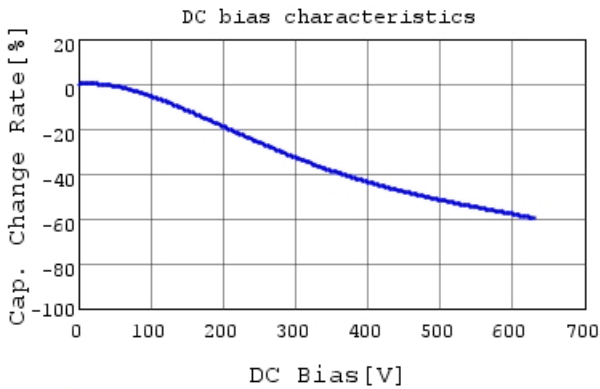
GC355DD72J104KX01 C-DC bias capchange, 25.0c
