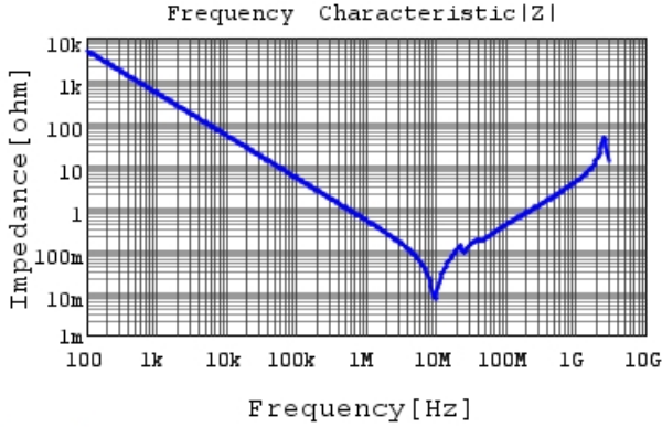
GC355DD72W334KX01 |Z| DCOV, 25degC
