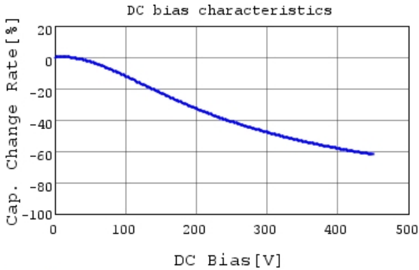
GC355DD72W334KX01 C-DC bias capchange, 25.0c
