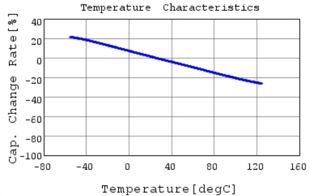
GC355DD72W334KX01 C-Temp. capchange, DCOV, 1
