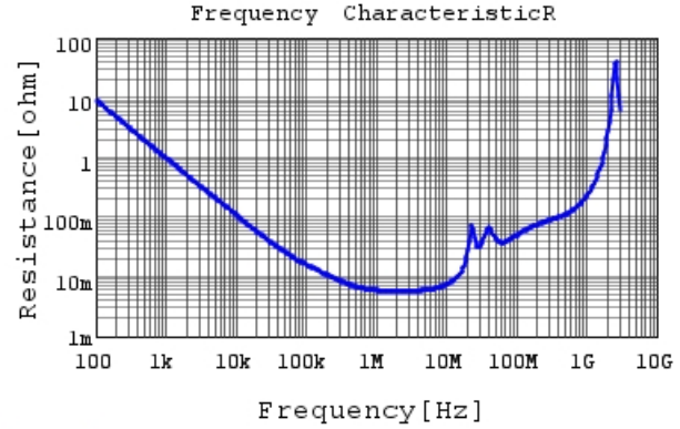
GC355DD72W334KX01 R DCOV, 25degC
