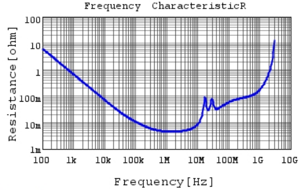
GC355DD72W474KX01 R DCOV, 25degC
