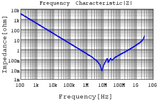
GC355DD72W474KX01 |Z| DCOV, 25degC
