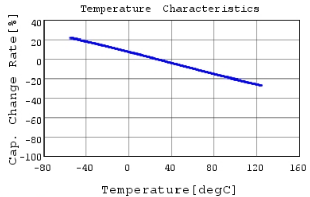
GC355DD72W474KX01 C-Temp. capchange, DCOV, 1
