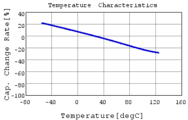
GC355XD72E105KX05 C-Temp. capchange, DC0V, 1
