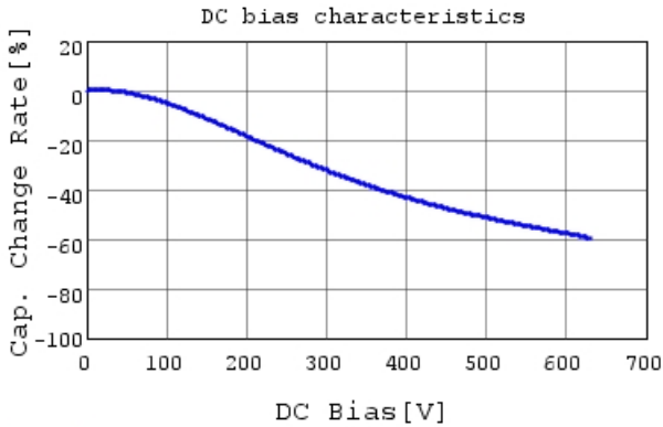
GC355XD72J224KX05 C-DC bias capchange, 25.0c
