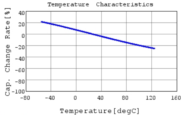
GC355XD72J224KX05 C-Temp. capchange, DC0V, 1
