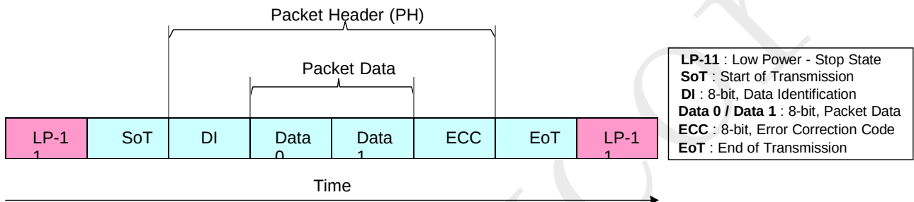
Figure 41 Short Packet (SPa) Structure
