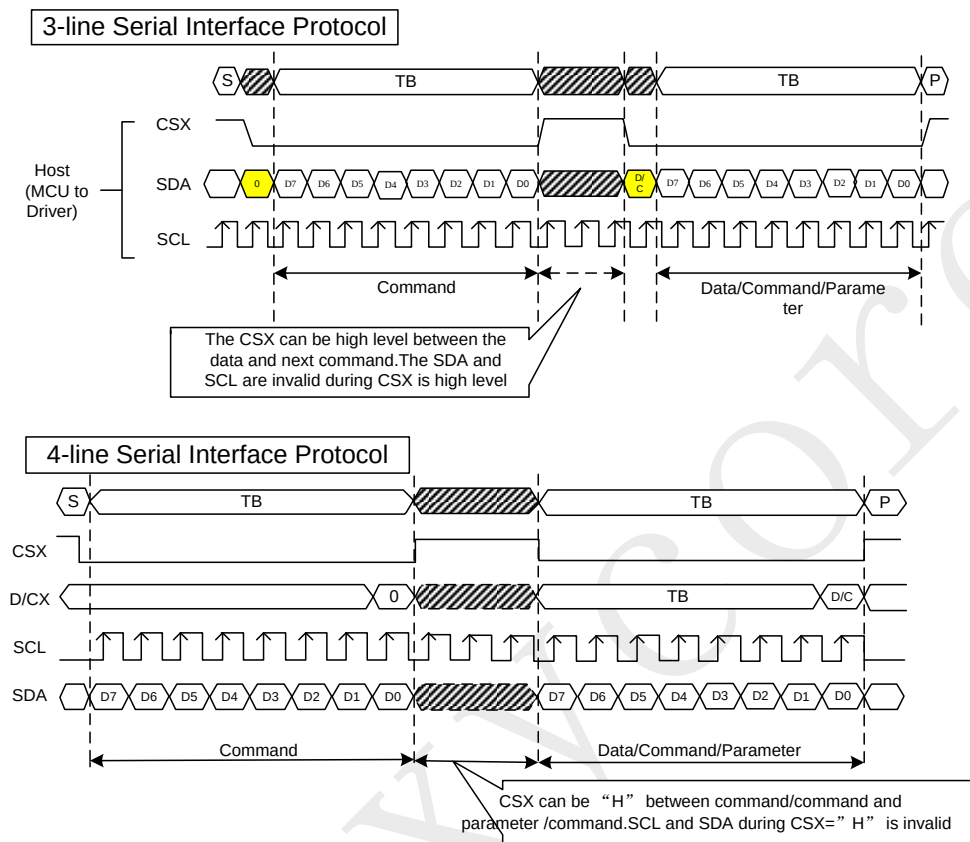
Figure 3 SPI protocol (SCL rising edge example)
