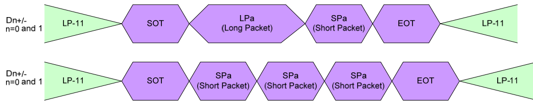
Figure 32 Multiple Packets in High-Speed Data Transmission – Examples
