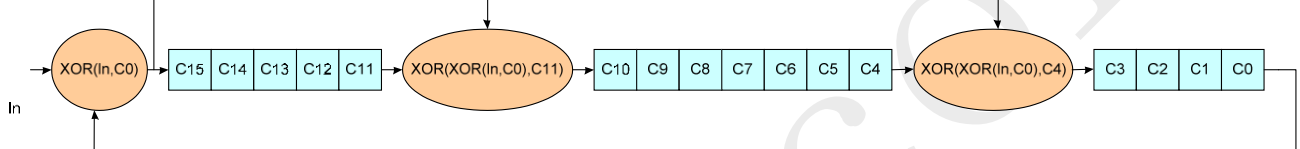
Figure 63 16-bit Cyclic Redundancy Check (CRC) Calculation
