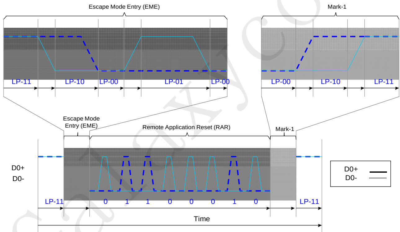
Figure 27 Remote Application Reset (RAR)
