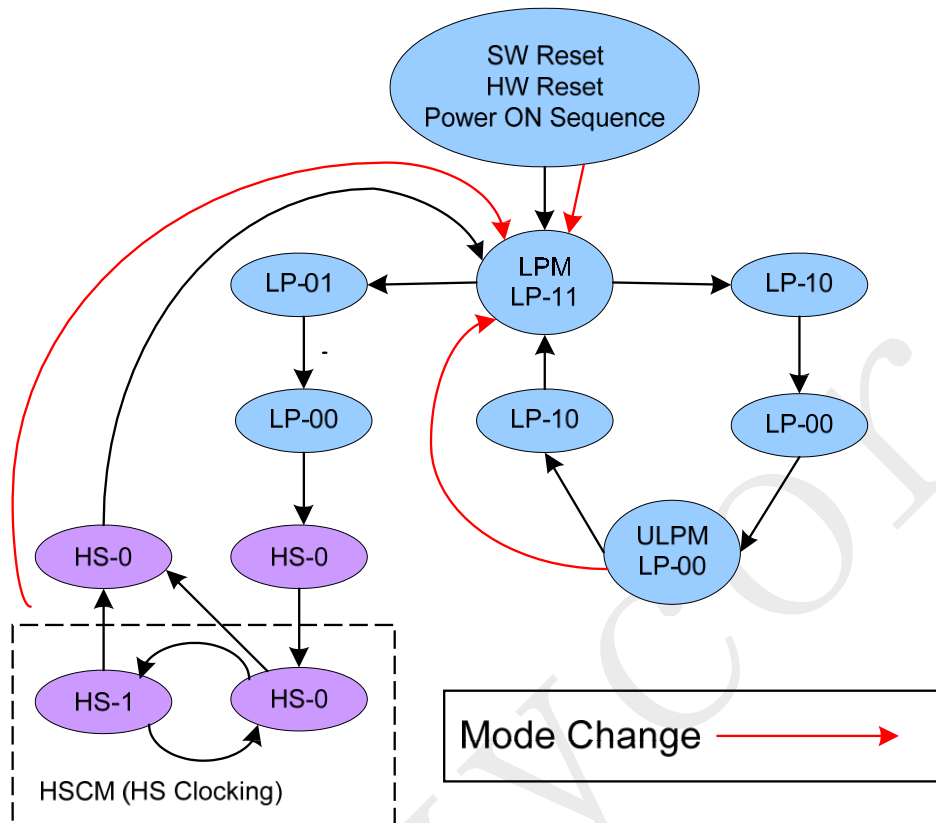
Figure 17 All Three Mode Changes to LPM on the Flow Chart
