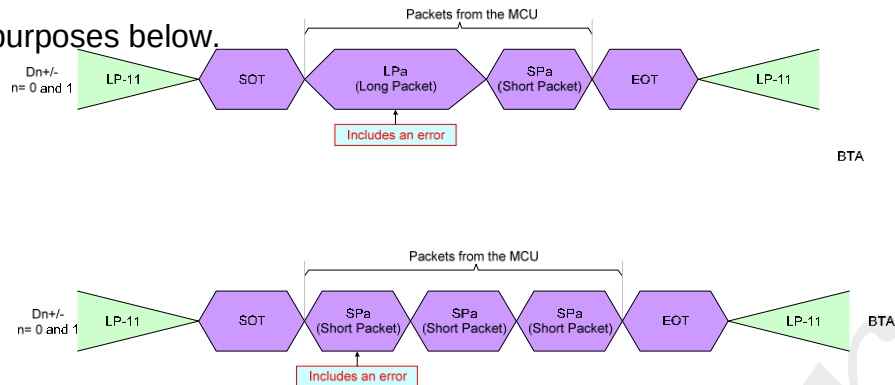
Figure 81 Errors Packets
