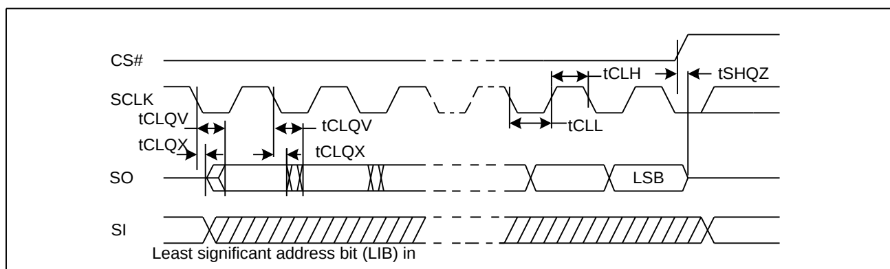
Figure 38. Output Timing
