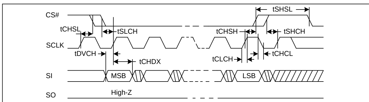
Figure 37. Input Timing
