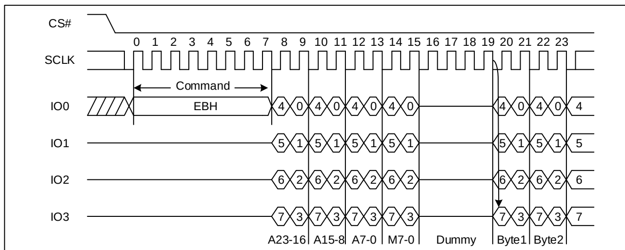
Figure 12. Quad I/O Fast Read Sequence Diagram ((M5-4) ≠ (1, 0))
