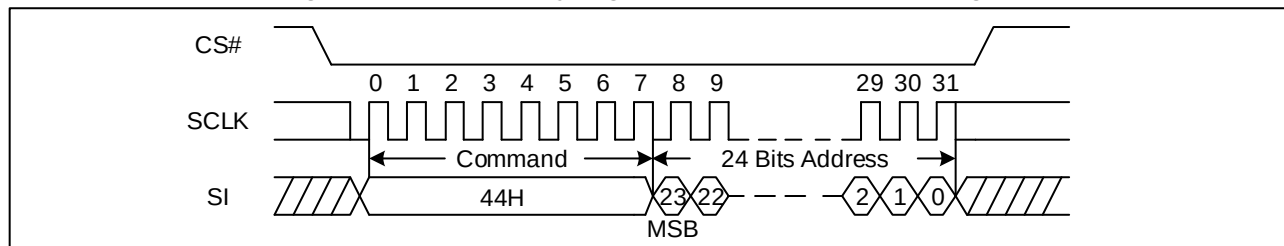
Figure 29. Erase Security Registers command Sequence Diagram
