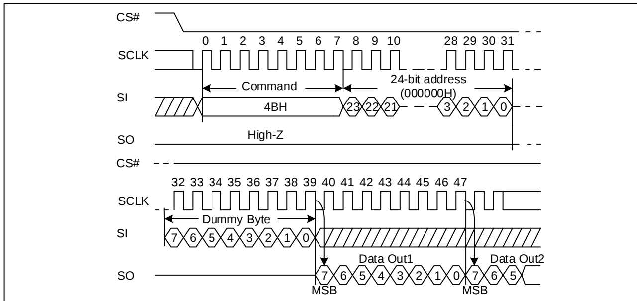
Figure 26. Read Unique ID Sequence Diagram
