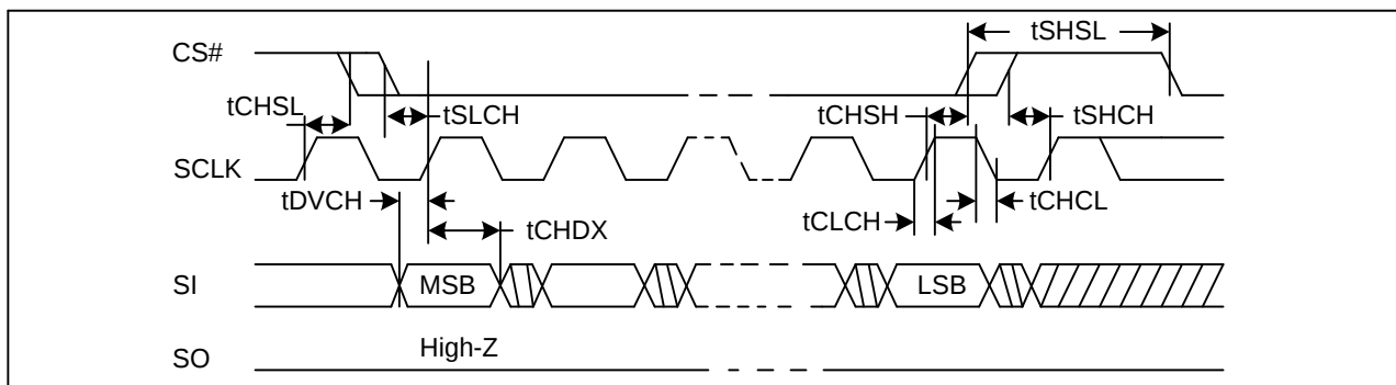
Figure 37. Input Timing
