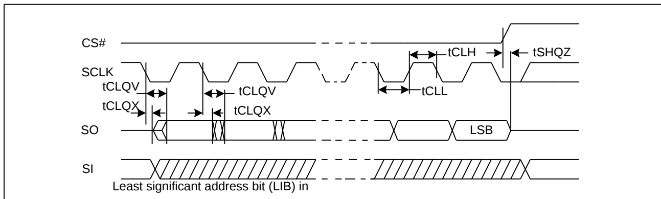
Figure 38. Output Timing
