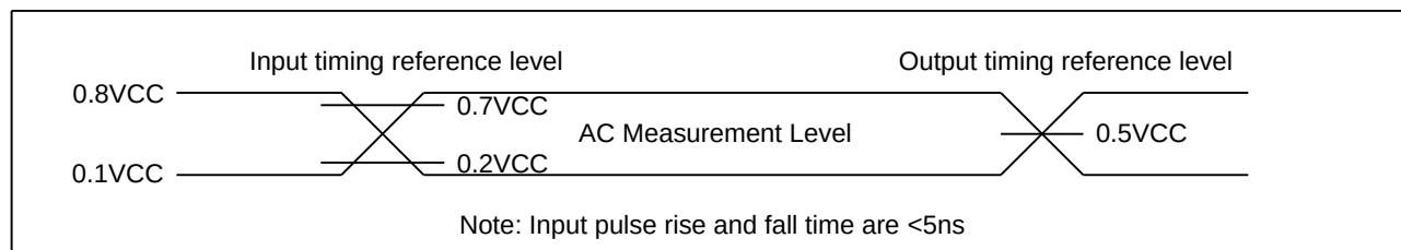
Figure21. Diagram Input Test Waveform and Measurement Level
