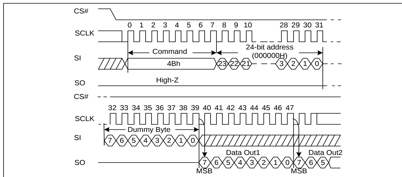
Figure 18. Read Unique ID Sequence Diagram
