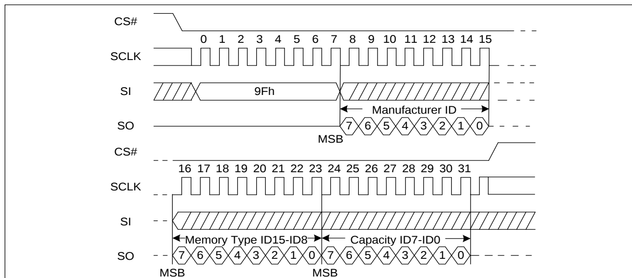
Figure 17. Read Identification ID Sequence Diagram
