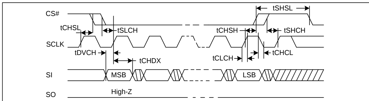
Figure 25. Input Timing
