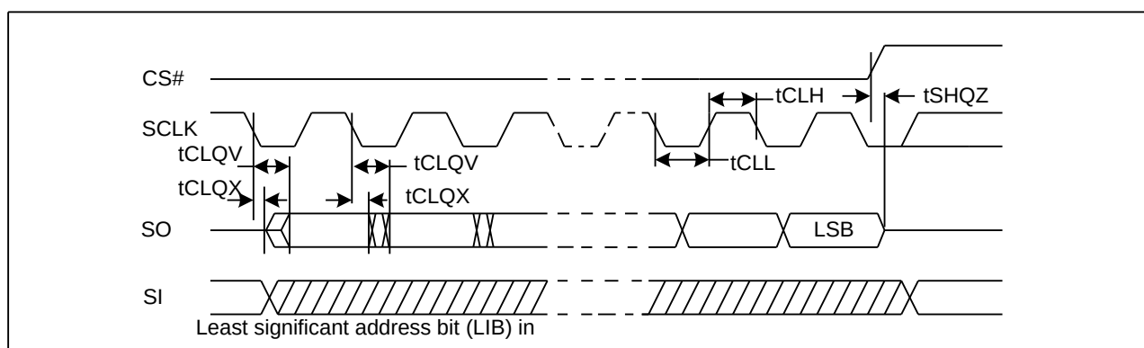
Figure23. Output Timing
