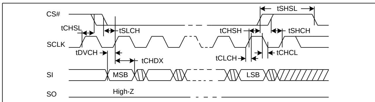
Figure22. Serial Input Timing
