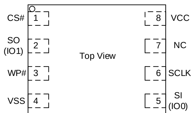
8 - LEAD USON
