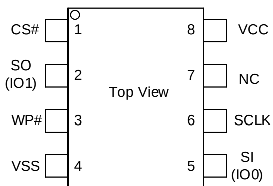
8 - LEAD SOP/TSSOP
