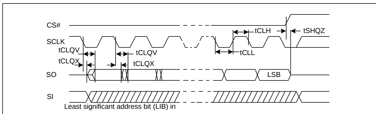
Figure 26. Output Timing
