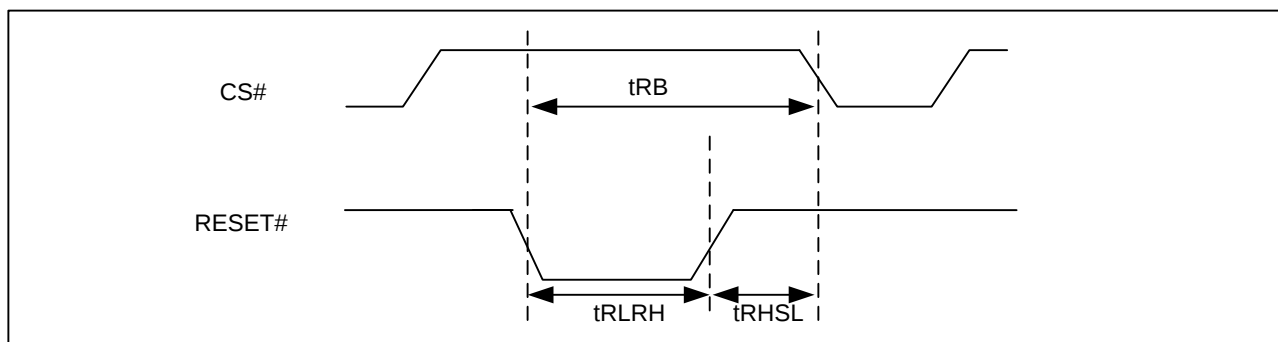
Figure 65 RESET Timing
