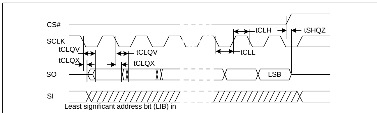
Figure 63. Output Timing
