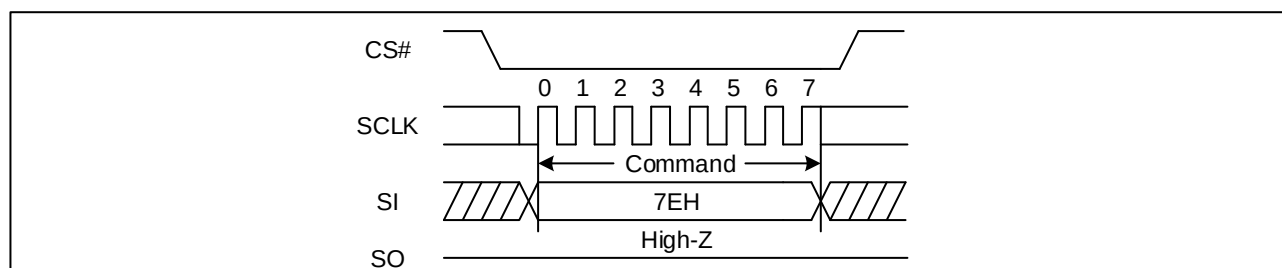
Figure 90 Global Block/Sector Lock Sequence Diagram (SPI)
