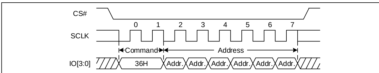
Figure 85 Individual Block/Sector Lock command Sequence Diagram (QPI)
