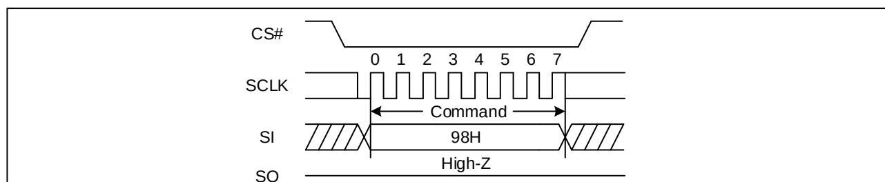
Figure 92 Global Block/Sector Unlock Sequence Diagram (SPI)
