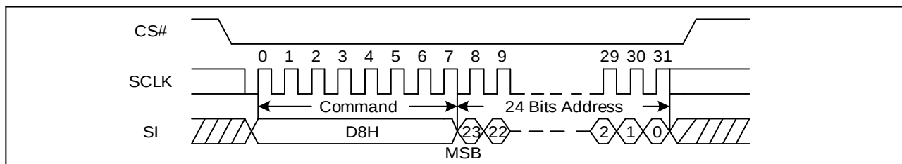
Figure 59 64KB Block Erase Sequence Diagram (SPI)
