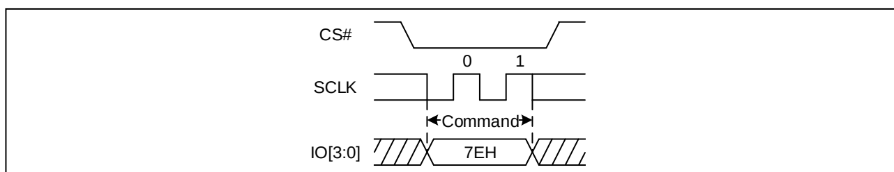
Figure 91 Global Block/Sector Lock Sequence Diagram (QPI)
