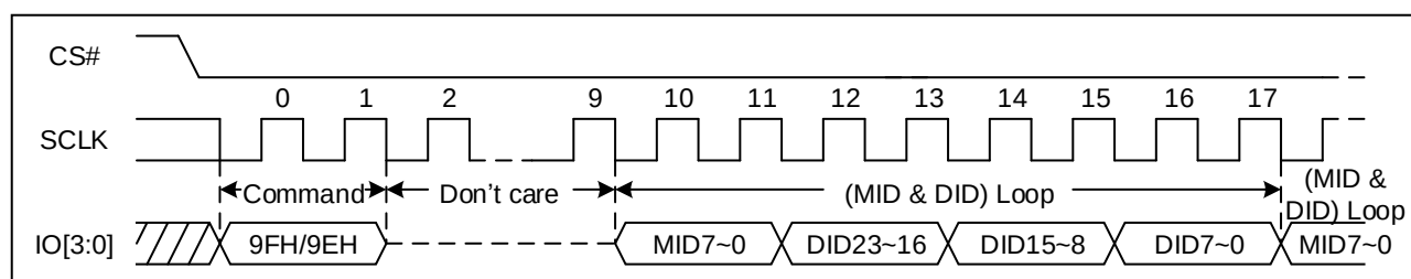
Figure 73 Read Identification ID Sequence Diagram (QPI, f_{SCLK} > 104\text{MHz} )
