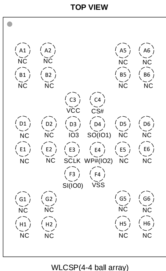
Figure 5 Connection Diagram for WLCSP (4-4 ball array) package
