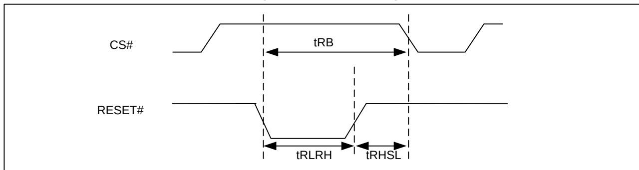
Figure 107. RESET Timing
