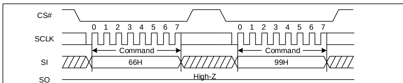
Figure 94 Enable Reset and Reset command Sequence Diagram (SPI)
