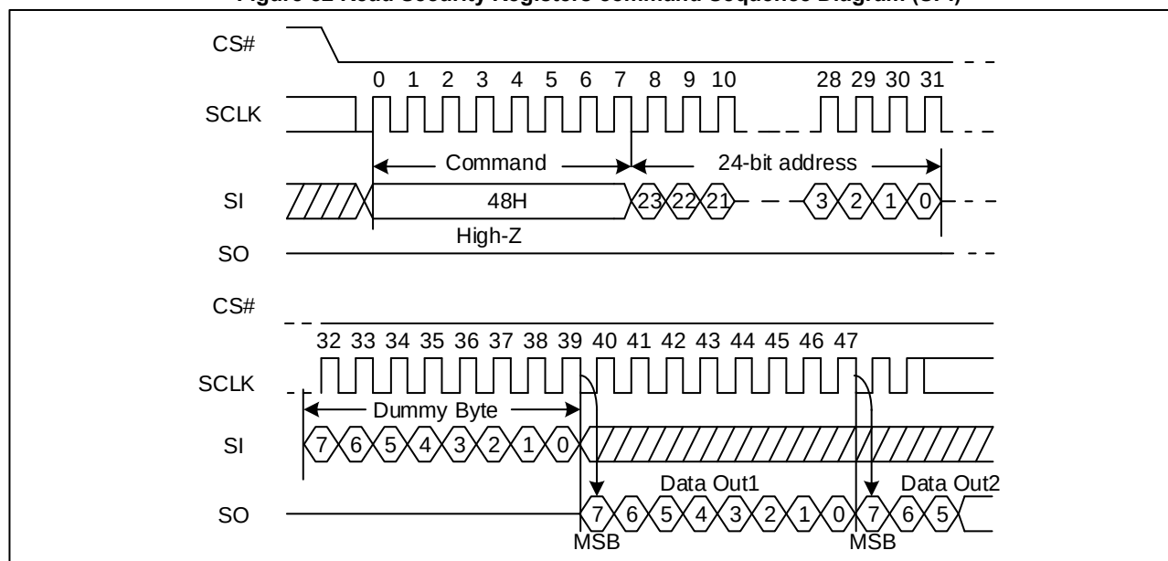
Figure 82 Read Security Registers command Sequence Diagram (SPI)
