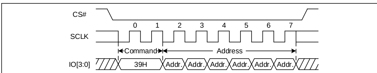
Figure 87 Individual Block/Sector Unlock command Sequence Diagram (QPI)
