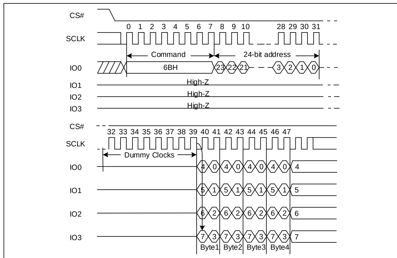
Figure 41 Quad Output Fast Read Sequence Diagram (SPI)
