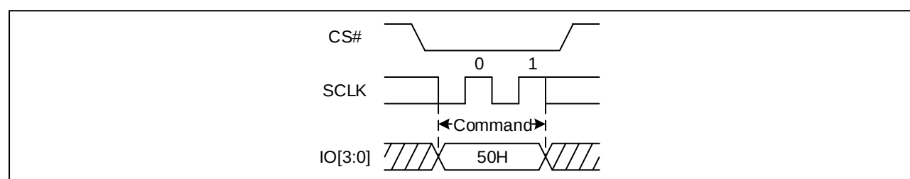
Figure 20 Write Enable for Volatile Status Register Sequence Diagram (QPI)
