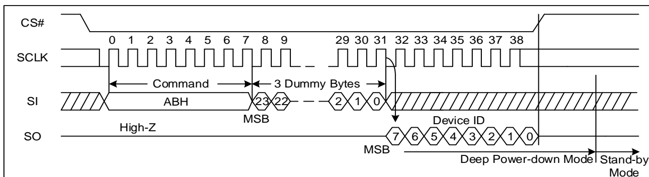
Figure 66. Release Power-Down/Read Device ID Sequence Diagram (SPI)
