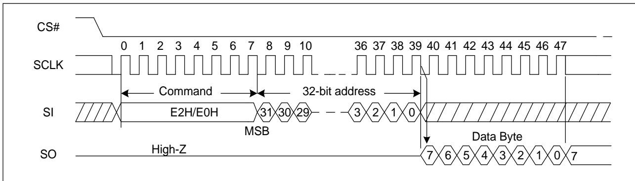
Figure 90 Read NL Register/VL Register Sequence Diagram (SPI)
