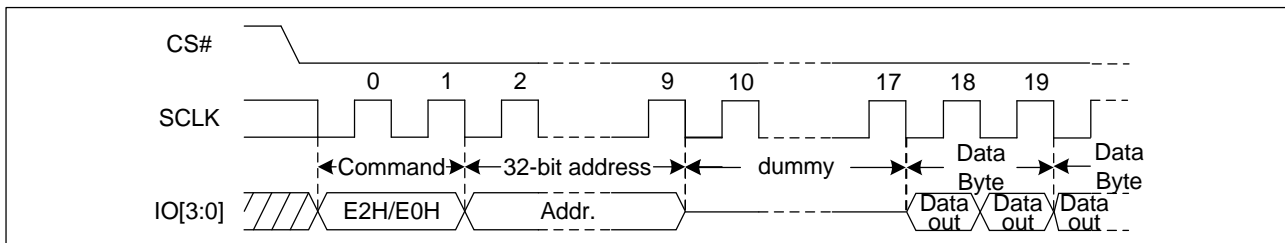
Figure 91 Read NL Register/VL Register Sequence (QPI)
