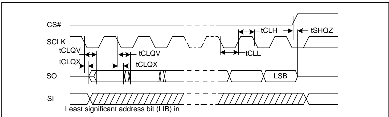
Figure 100. Output Timing
