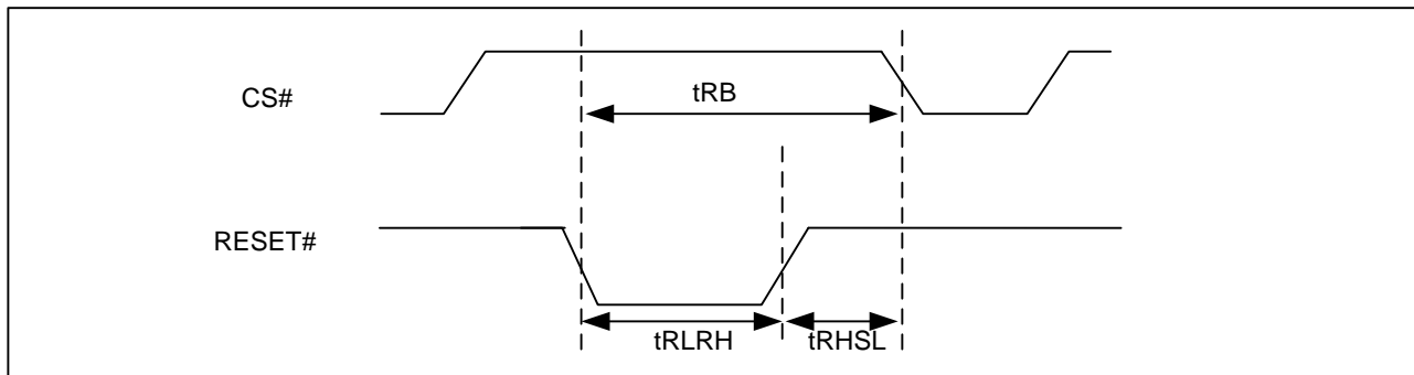
Figure 103. RESET Timing
