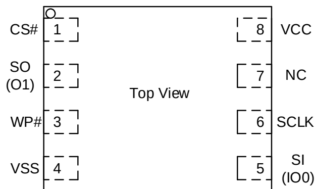
8 - LEAD USON
