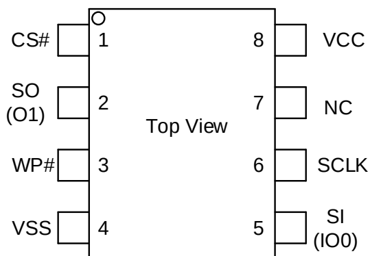
8 - LEAD VSOP/SOP/DIP
