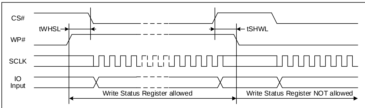
Figure 27. WP# Timing
