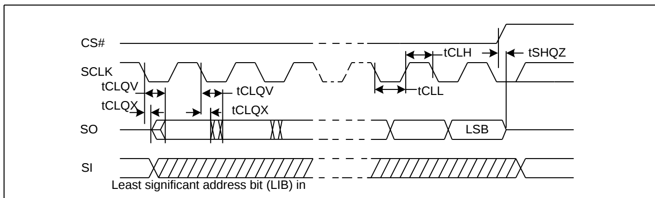
Figure 26. Output Timing
