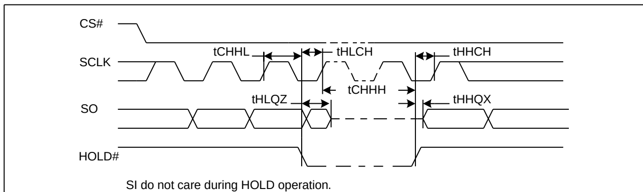
Figure 73. Hold Timing
