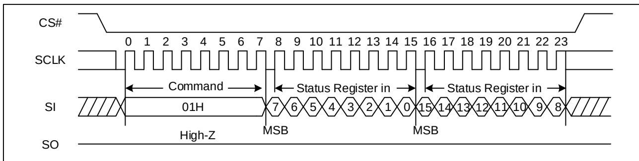
Figure 13. Write Status Register-1&2 Sequence Diagram (SPI)
