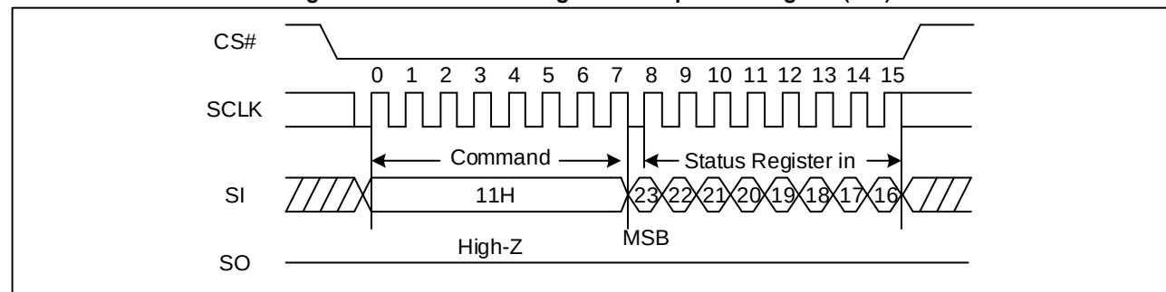
Figure 15. Write Status Register-3 Sequence Diagram (SPI)
