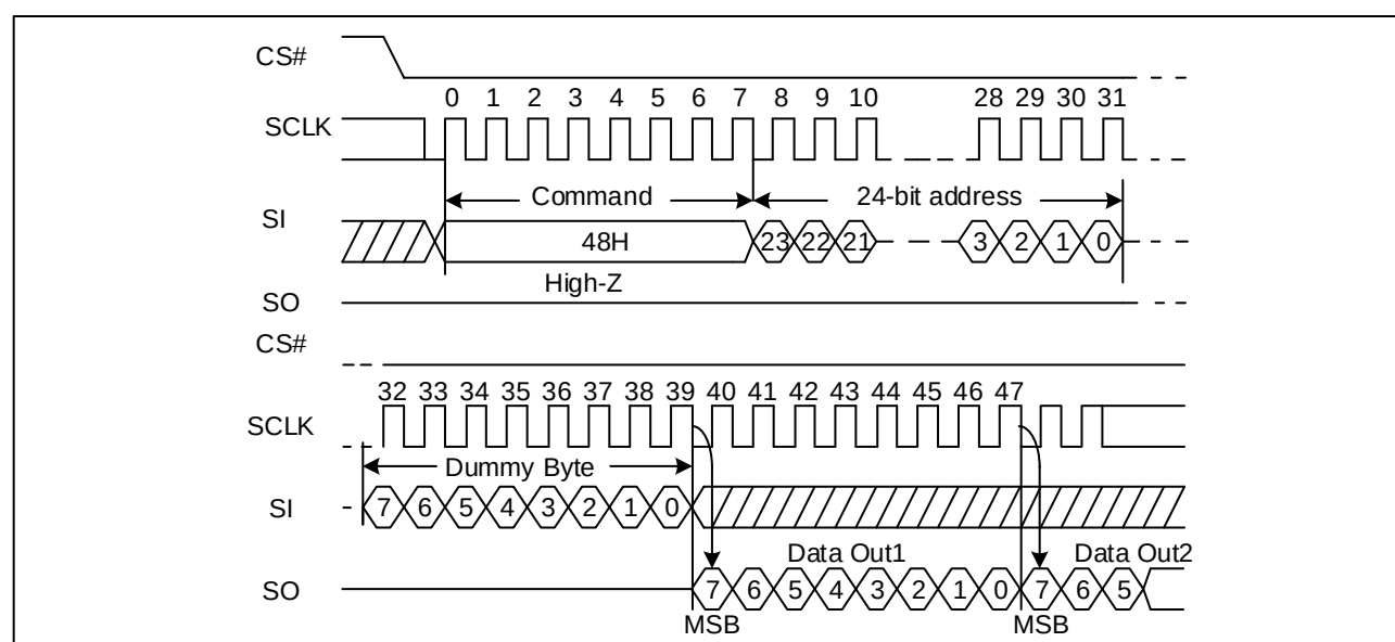
Figure 50. Read Security Registers command Sequence Diagram
