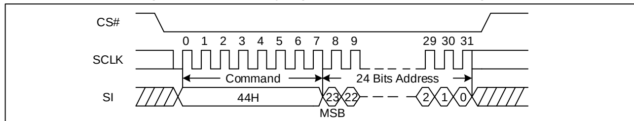
Figure 27. Erase Security Registers command Sequence Diagram
