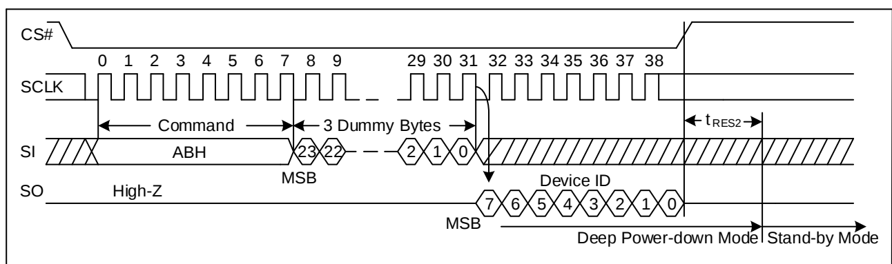
Figure 25. Release Power-Down/Read Device ID Sequence Diagram
