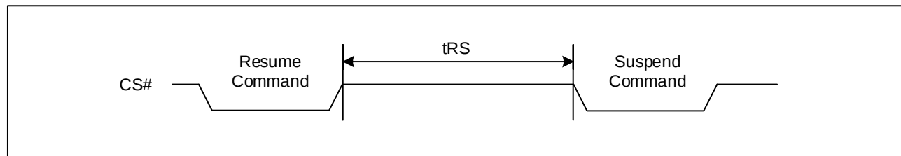
Figure 43. Resume to Suspend Timing
