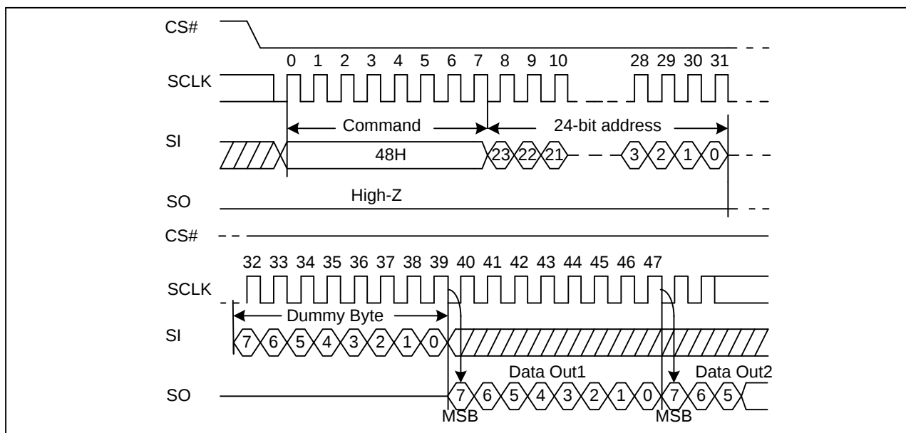
Figure 35. Read Security Registers command Sequence Diagram
