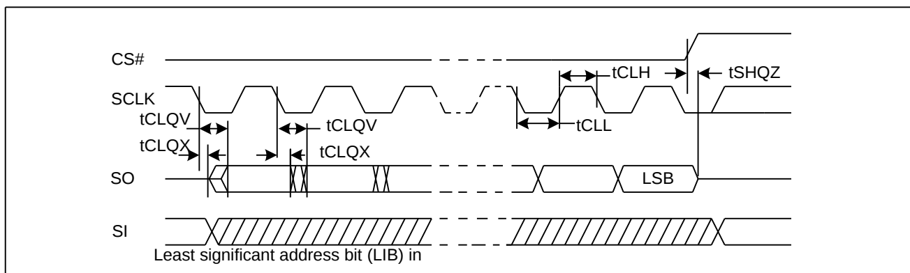
Figure 42. Output Timing
