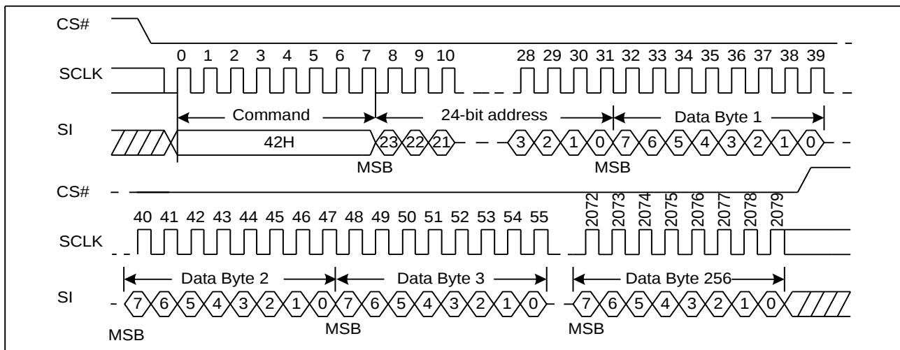
Figure 34. Program Security Registers command Sequence Diagram
