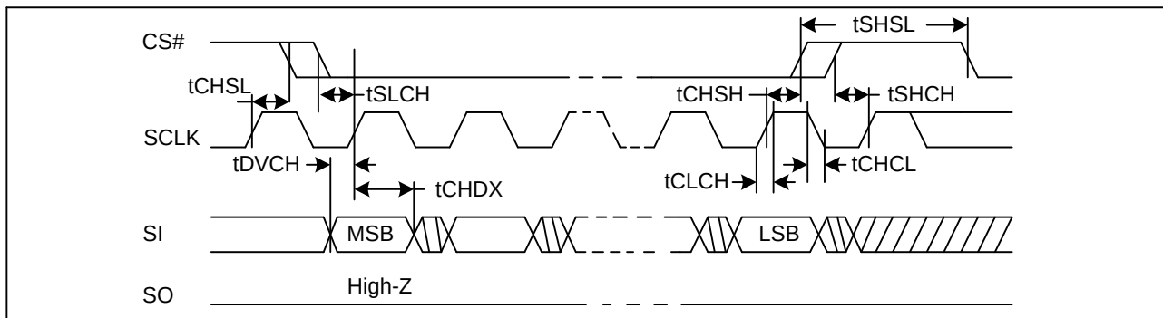
Figure 62. Input Timing
