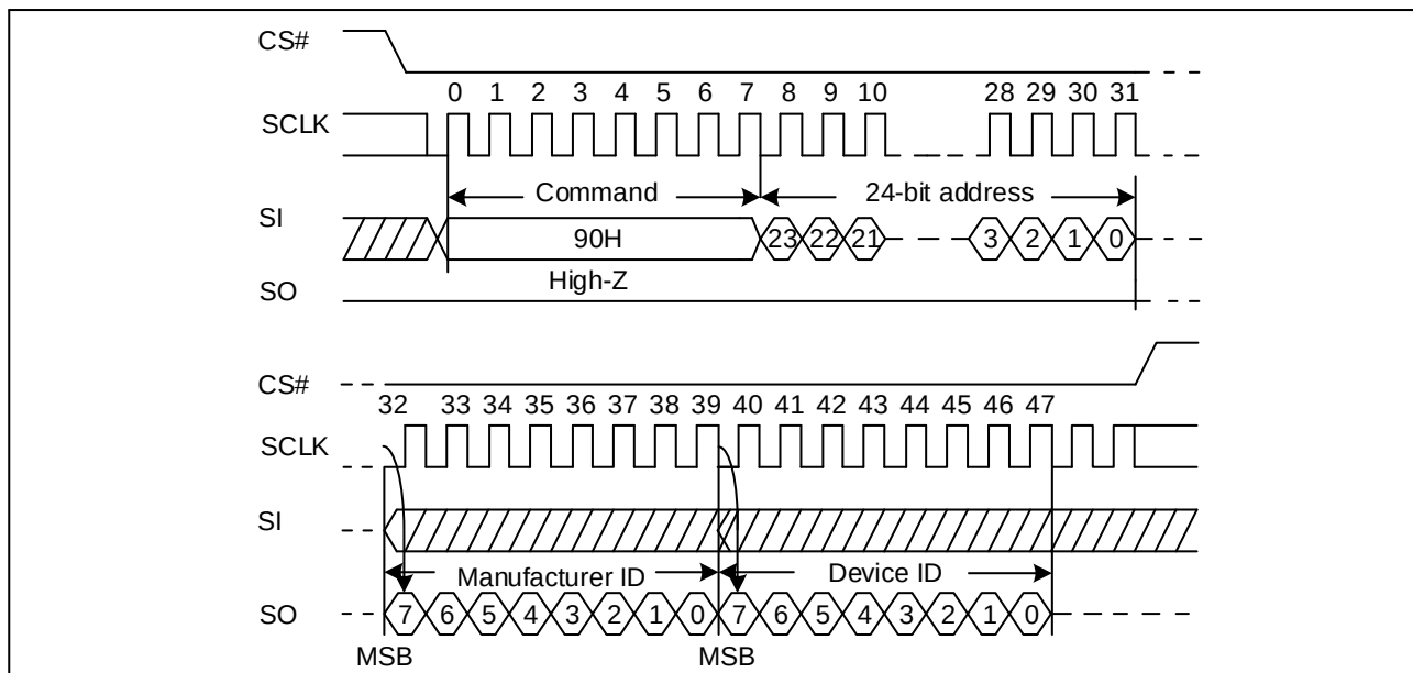
Figure 34. Read Manufacturer ID/ Device ID Sequence Diagram (SPI)
