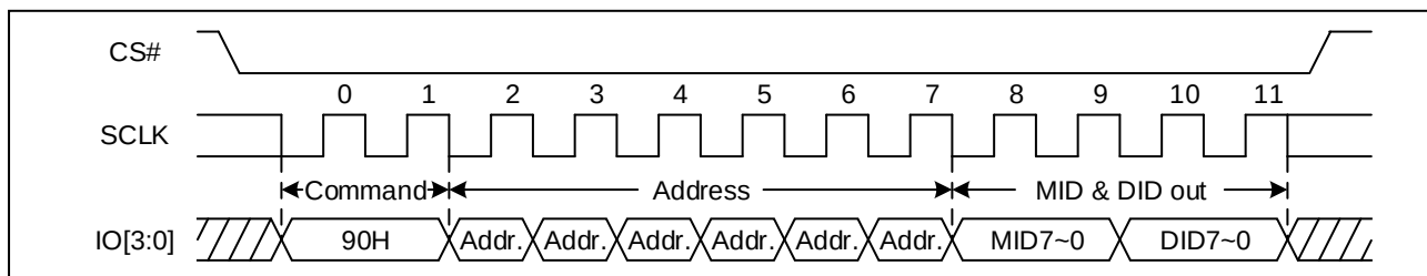
Figure 35. Read Manufacturer ID/ Device ID Sequence Diagram (QPI)
