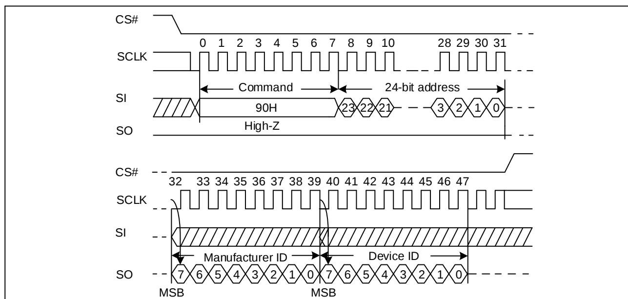
Figure 44. Read Manufacturer ID/ Device ID Sequence Diagram (SPI)
