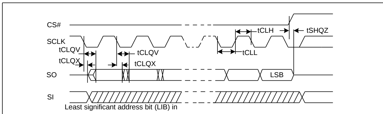
Figure 72. Output Timing
