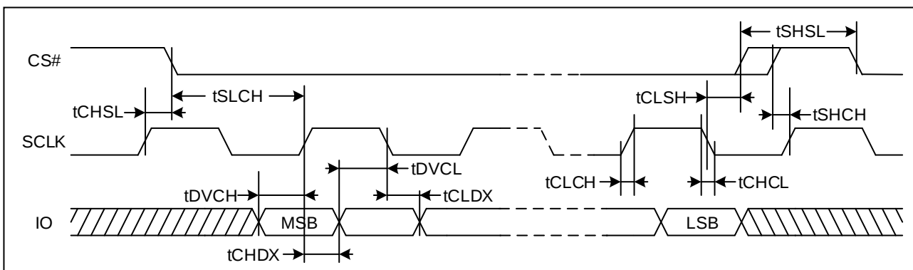
Figure 73. Serial Input Timing (DTR)
