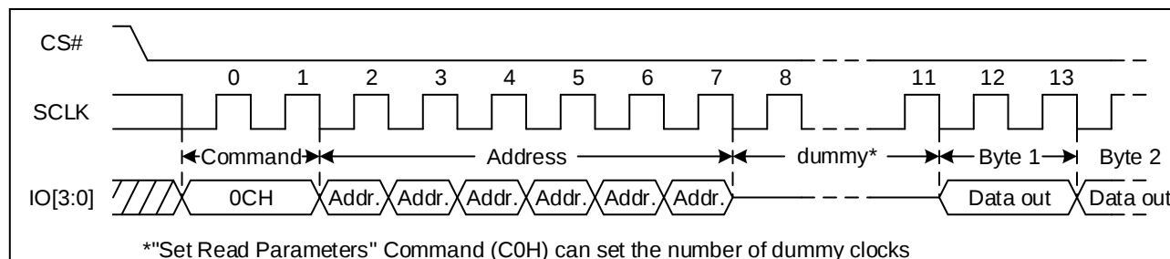
Figure 27. Burst Read with Wrap command Sequence Diagram
