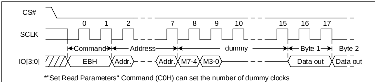
Figure 25. Quad I/O Fast Read Sequence Diagram (QPI, M5-4 ≠ (1, 0))
