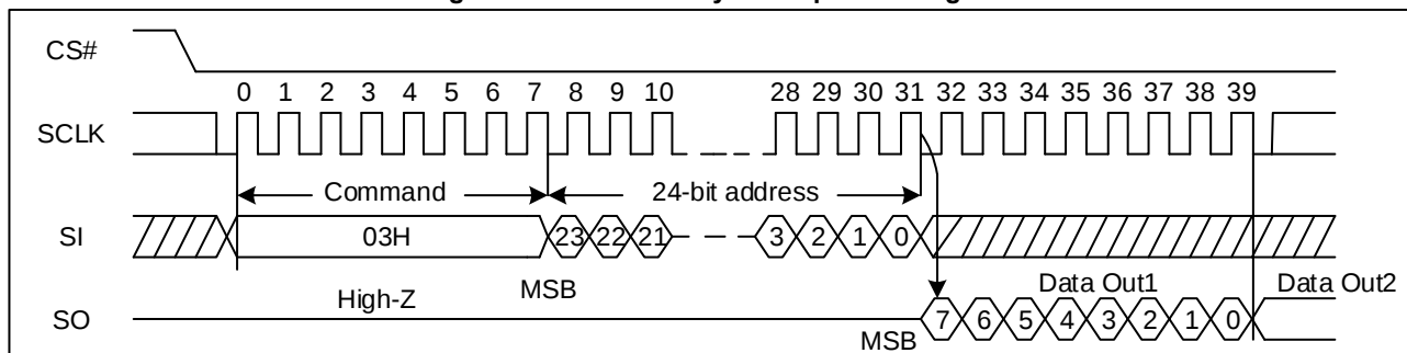
Figure 17. Read Data Bytes Sequence Diagram
