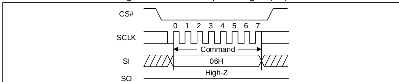
Figure 5. Write Enable Sequence Diagram (SPI)
