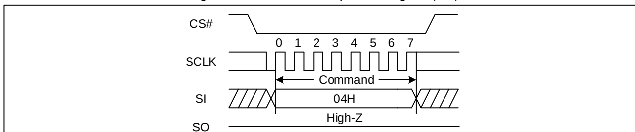
Figure 7. Write Disable Sequence Diagram (SPI)
