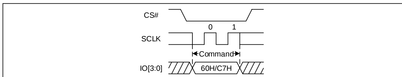
Figure 43. Chip Erase Sequence Diagram (QPI)
