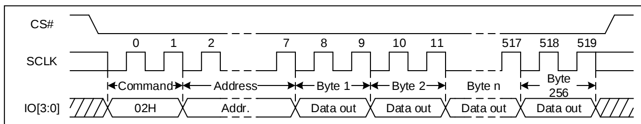
Figure 34. Page Program Sequence Diagram (QPI)
