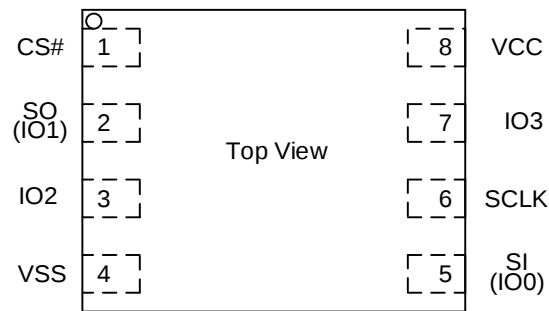
8 - LEAD USON/WSN
