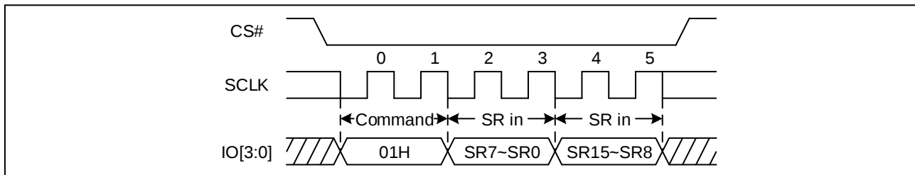
Figure 12. Write Status Register-1&2 Sequence Diagram (QPI)
