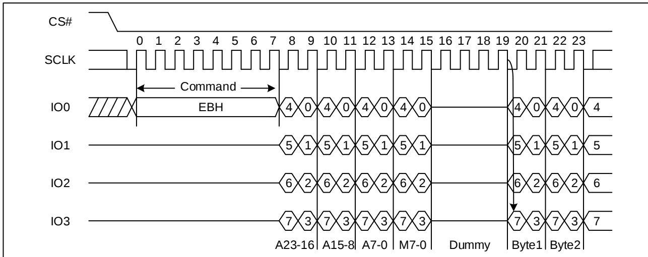
Figure 24. Quad I/O Fast Read Sequence Diagram (SPI, M5-4 ≠ (1, 0))
