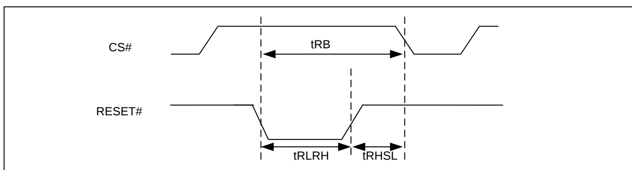
Figure 76 RESET Timing
