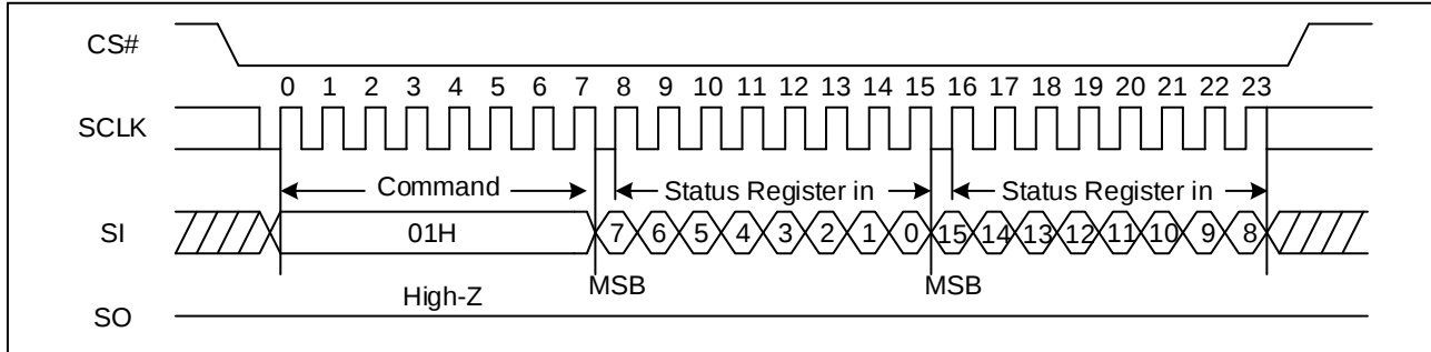
Figure 11. Write Status Register-1&2 Sequence Diagram (SPI)
