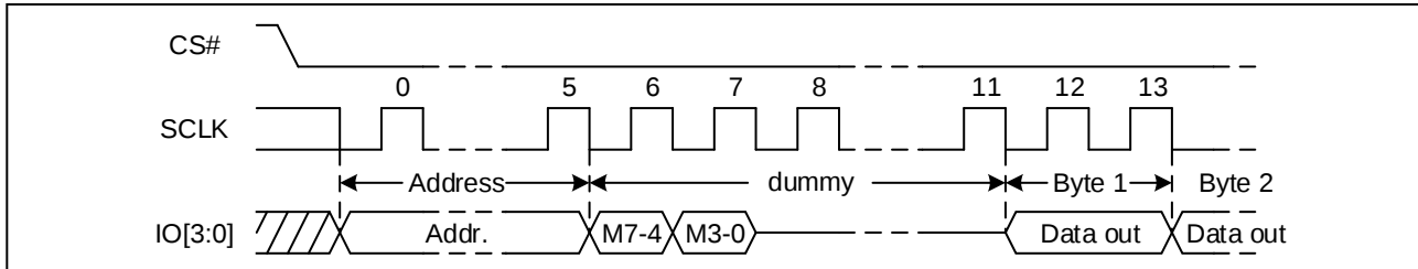
Figure 26 Quad I/O Fast Read Sequence Diagram (M5-4 = (1, 0))
