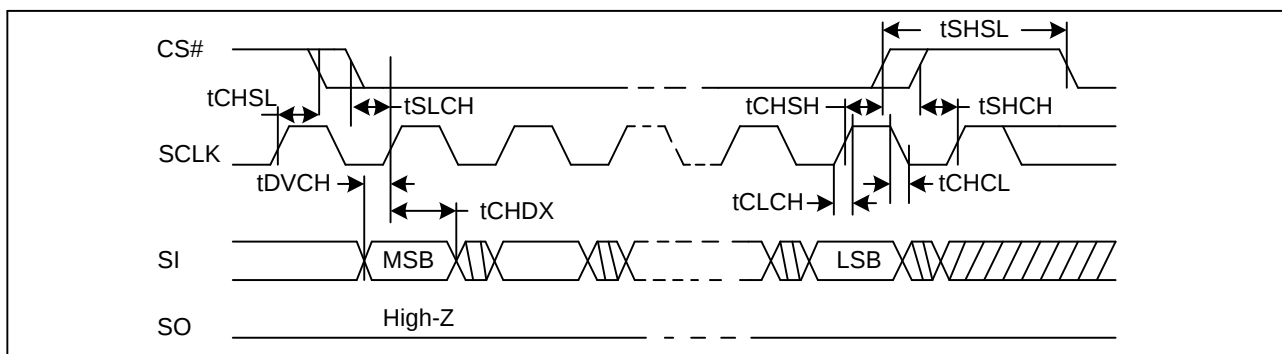
Figure 71. Input Timing
