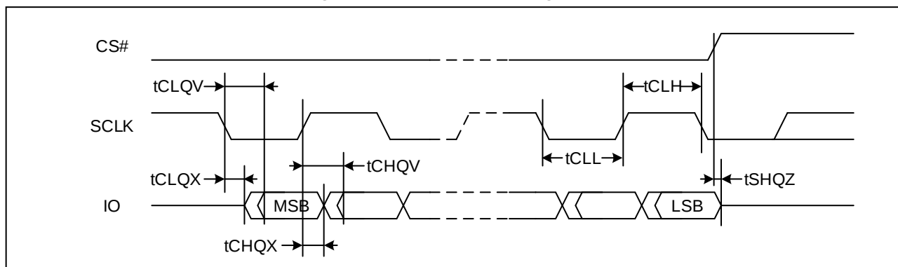
Figure 74. Serial Output Timing (DTR)
