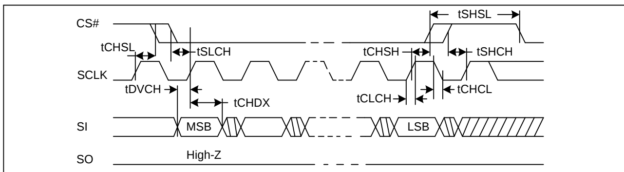
Figure 67. Input Timing
