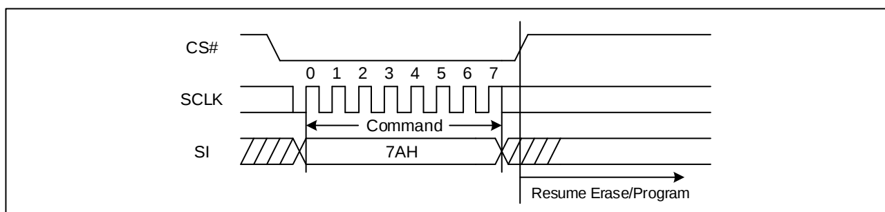
Figure 52. Program/Erase Resume Sequence Diagram (SPI)
