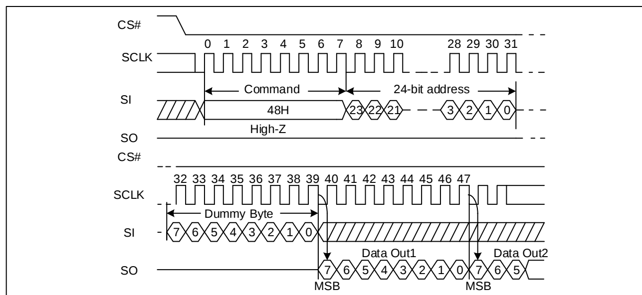
Figure 47. Read Security Registers command Sequence Diagram
